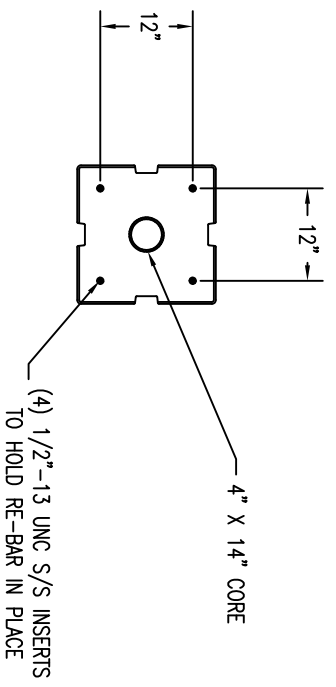
3 BOTTOM VIEW
