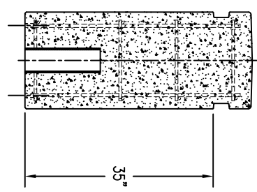
4 CROSS SECTION
