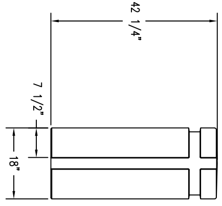
2 ELEVATION VIEW
