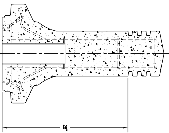
4 CROSS SECTION
