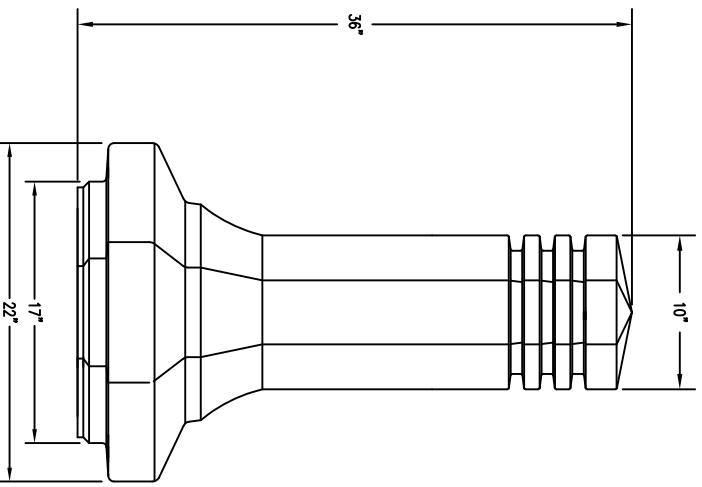
1 TOP VIEW
