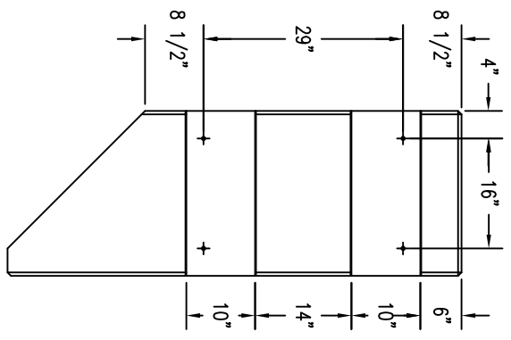
3 BOTTOM VIEW
